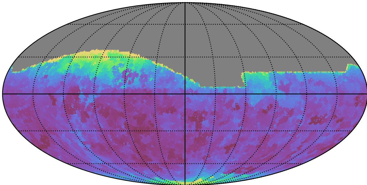
ddf_loaded_fl4_v3.4_10yrs All sky i band: Min seeingEff
