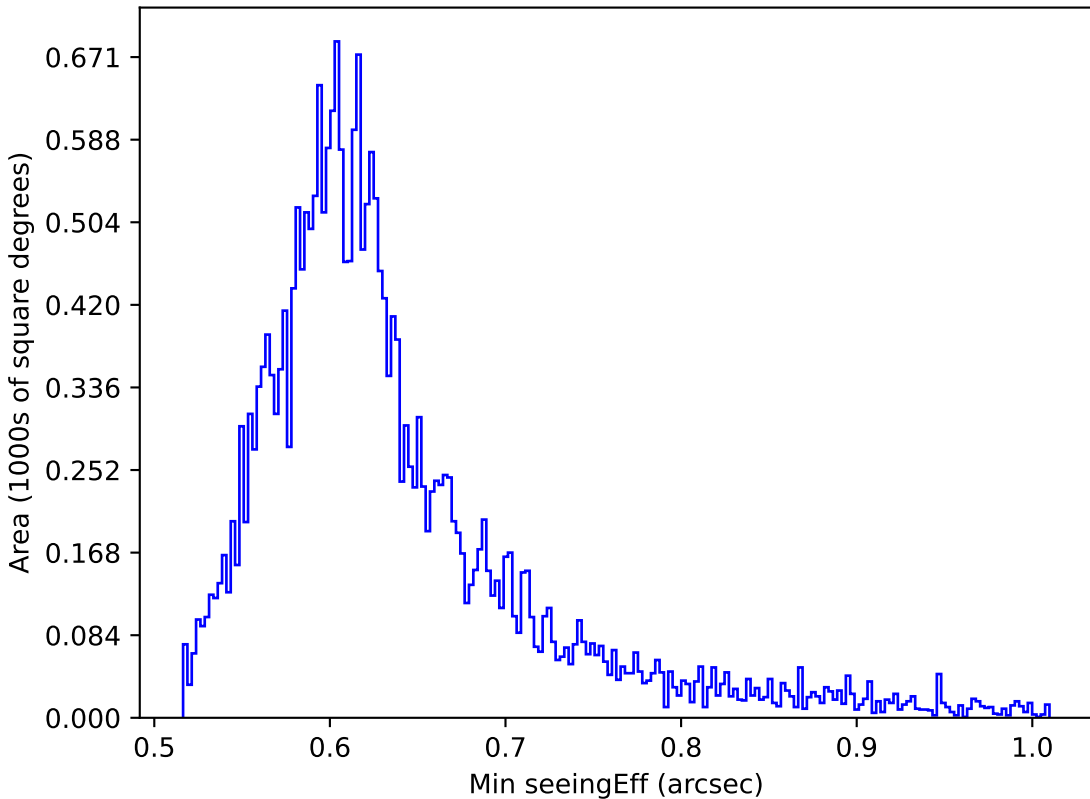
ddf_loaded_fl4_v3.4_10yrs All sky i band: Min seeingEff
