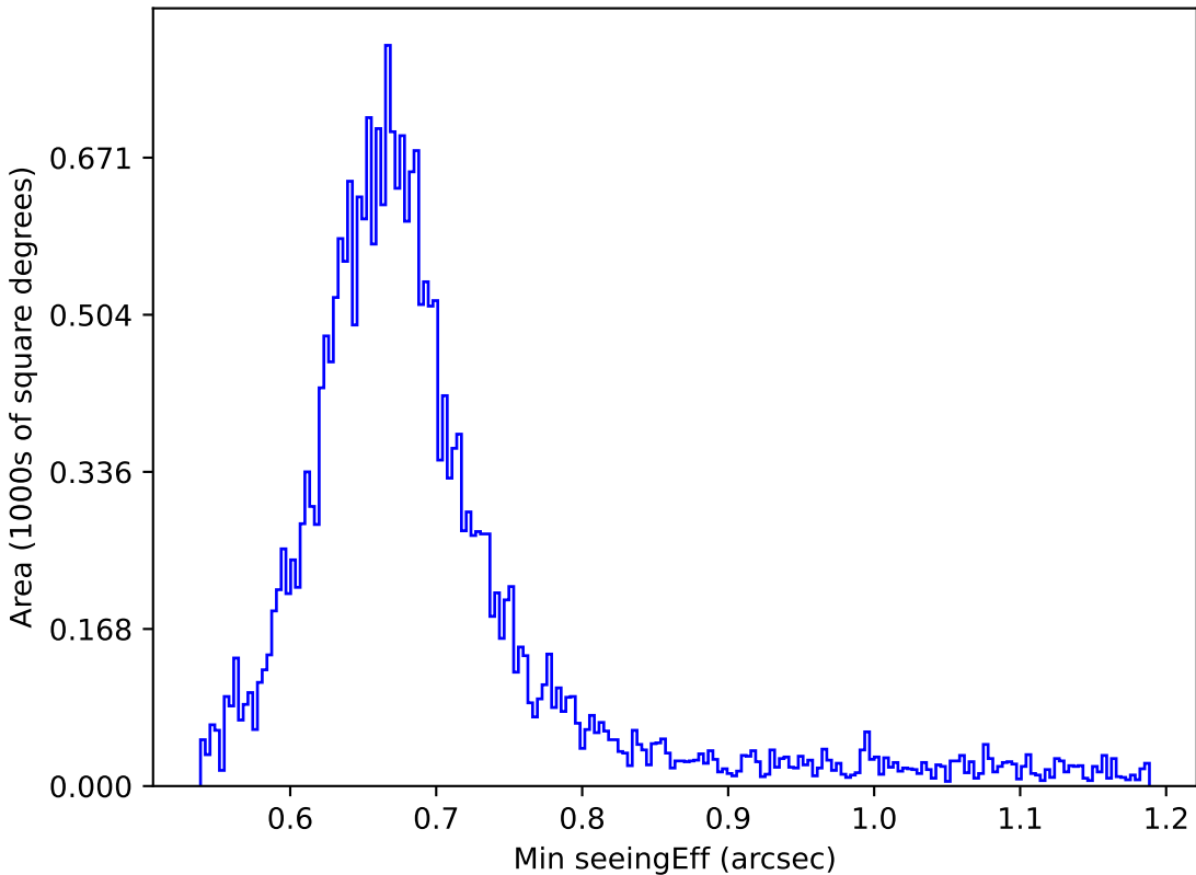
ddf_loaded_fl4_v3.4_10yrs All sky g band: Min seeingEff
