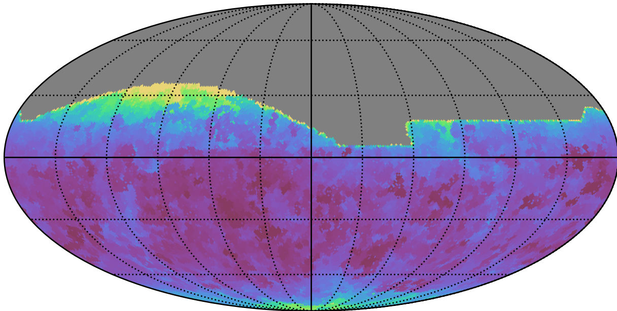
ddf_loaded_fl4_v3.4_10yrs All sky all bands: Min seeingEff
