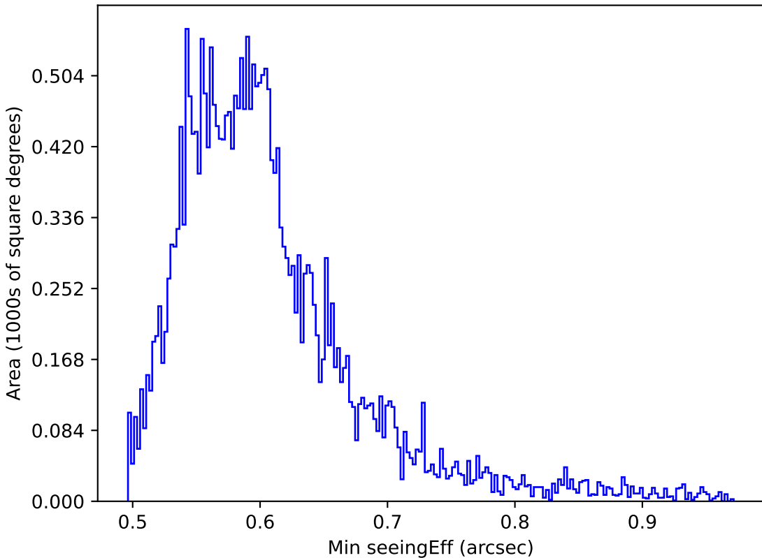
ddf_loaded_fl4_v3.4_10yrs All sky all bands: Min seeingEff
