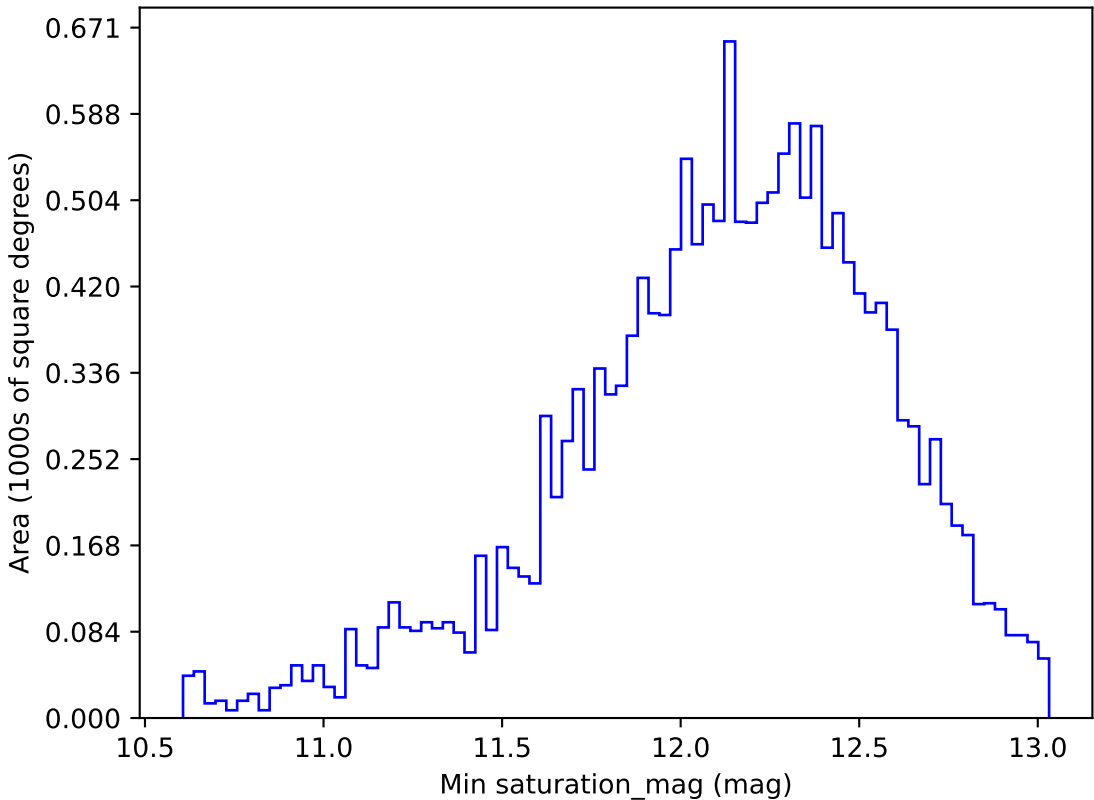
ddf_loaded_fl4_v3.4_10yrs WFD z band: Min saturation_mag
