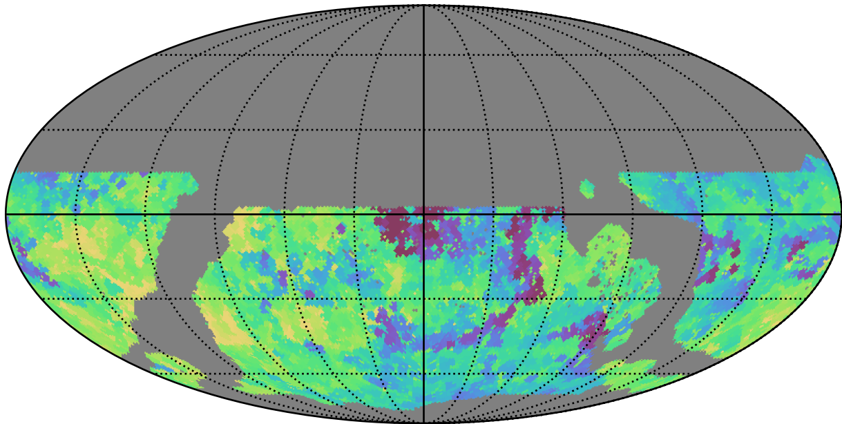
ddf_loaded_fl4_v3.4_10yrs WFD y band: Min saturation_mag
