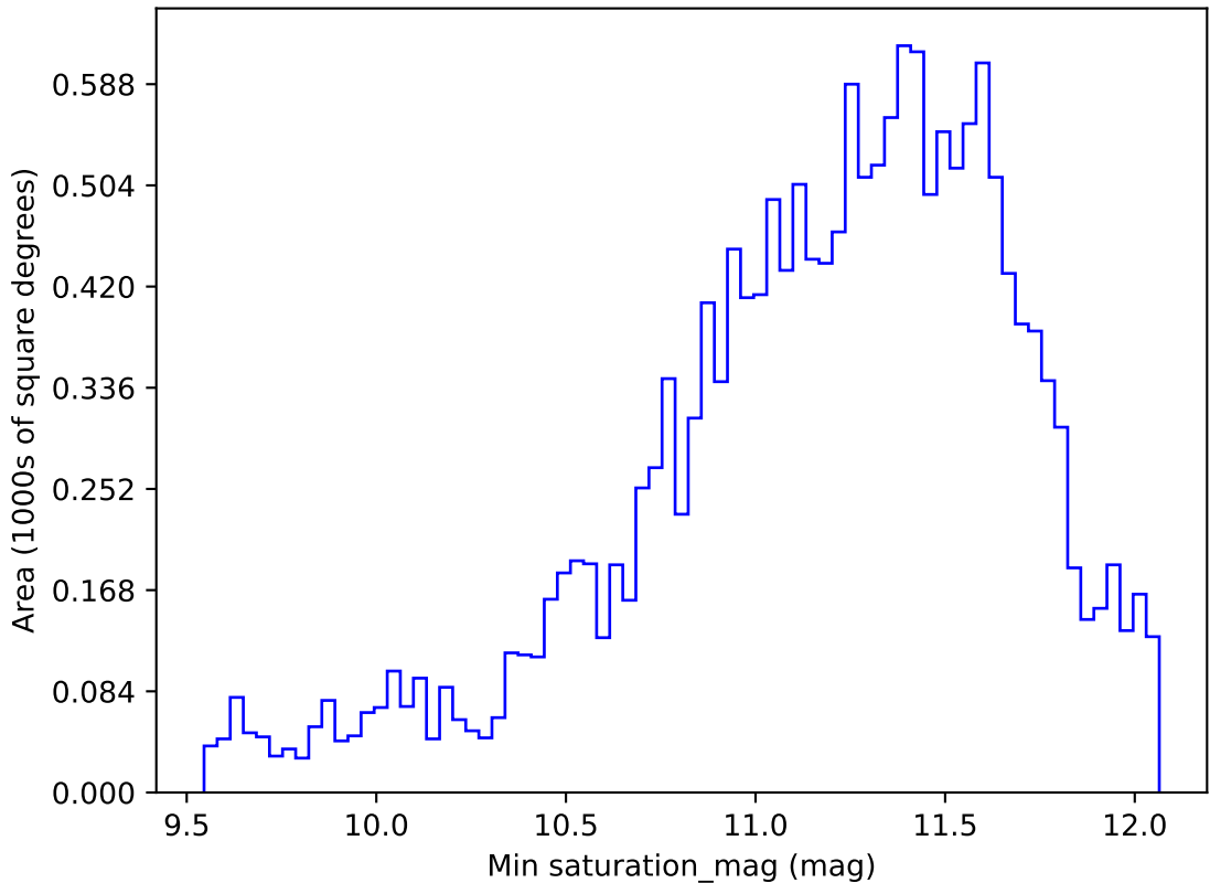
ddf_loaded_fl4_v3.4_10yrs WFD y band: Min saturation_mag
