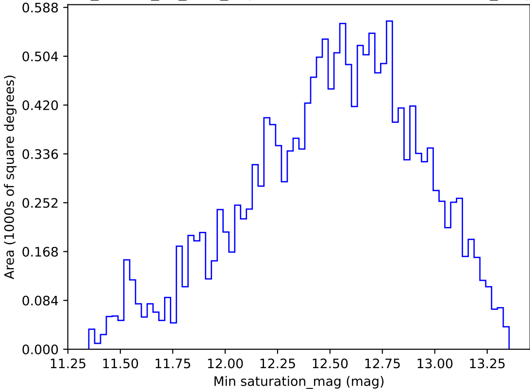
ddf_loaded_fl4_v3.4_10yrs WFD r band: Min saturation_mag
