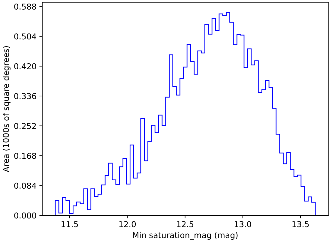
ddf_loaded_fl4_v3.4_10yrs WFD g band: Min saturation_mag
