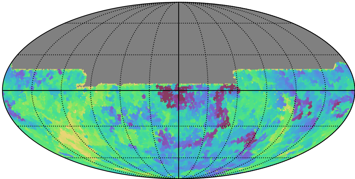
ddf_loaded_fl4_v3.4_10yrs All sky y band: Min saturation_mag
