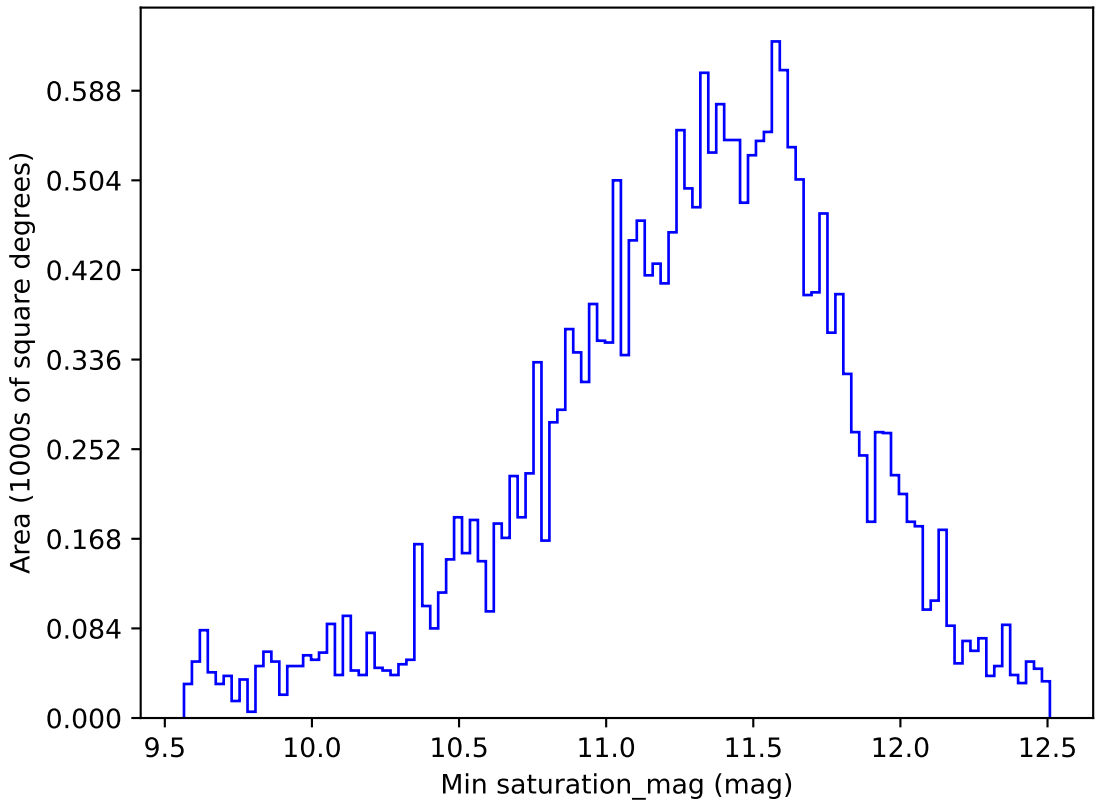
ddf_loaded_fl4_v3.4_10yrs All sky y band: Min saturation_mag
