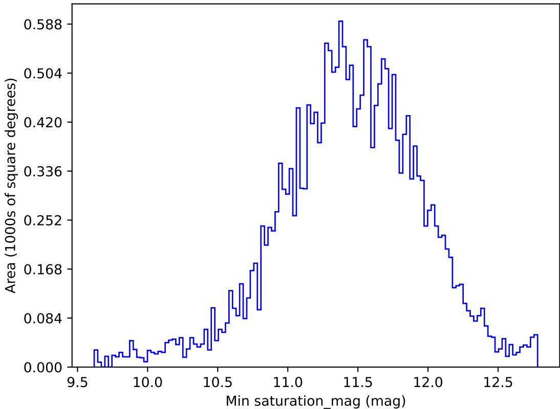
ddf_loaded_fl4_v3.4_10yrs All sky u band: Min saturation_mag
