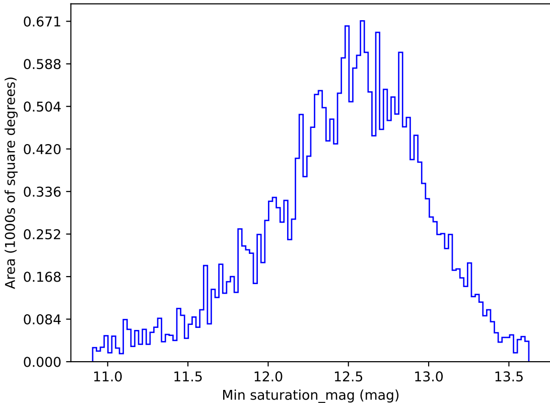
ddf_loaded_fl4_v3.4_10yrs All sky i band: Min saturation_mag
