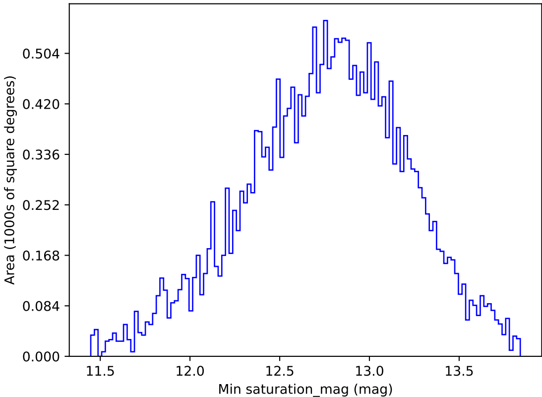
ddf_loaded_fl4_v3.4_10yrs All sky g band: Min saturation_mag
