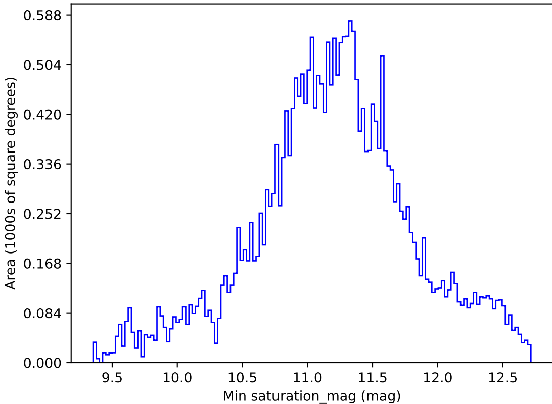
ddf_loaded_fl4_v3.4_10yrs All sky all bands: Min saturation_mag
