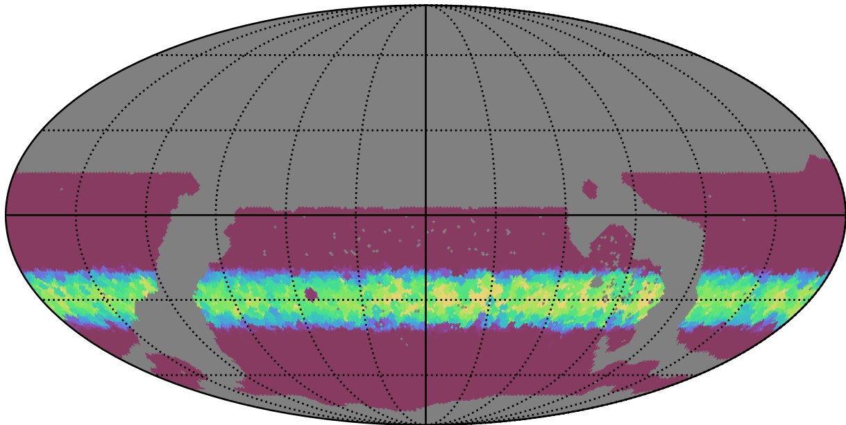
ddf_loaded_fl4_v3.4_10yrs WFD z band: Min normairmass
