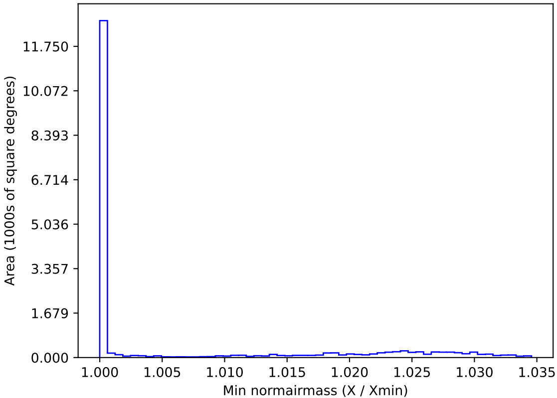
ddf_loaded_fl4_v3.4_10yrs WFD z band: Min normairmass
