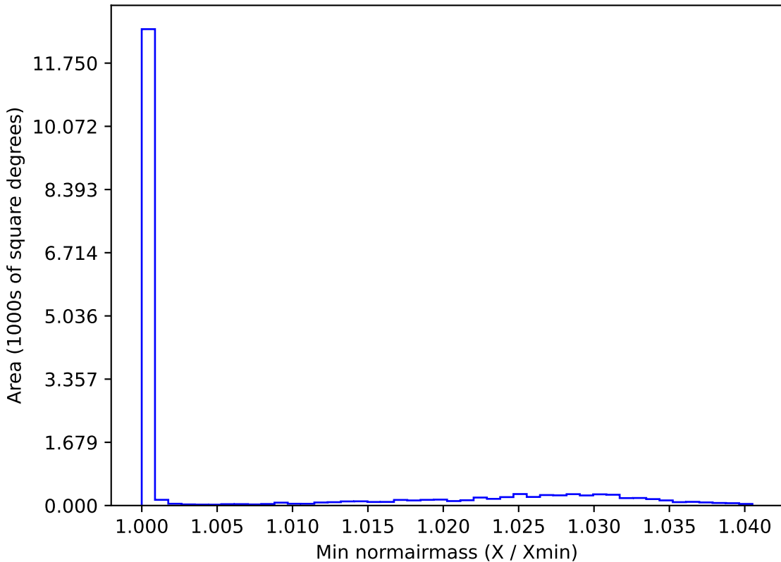
ddf_loaded_fl4_v3.4_10yrs WFD y band: Min normairmass
