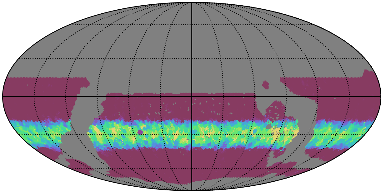
ddf_loaded_fl4_v3.4_10yrs WFD u band: Min normairmass
