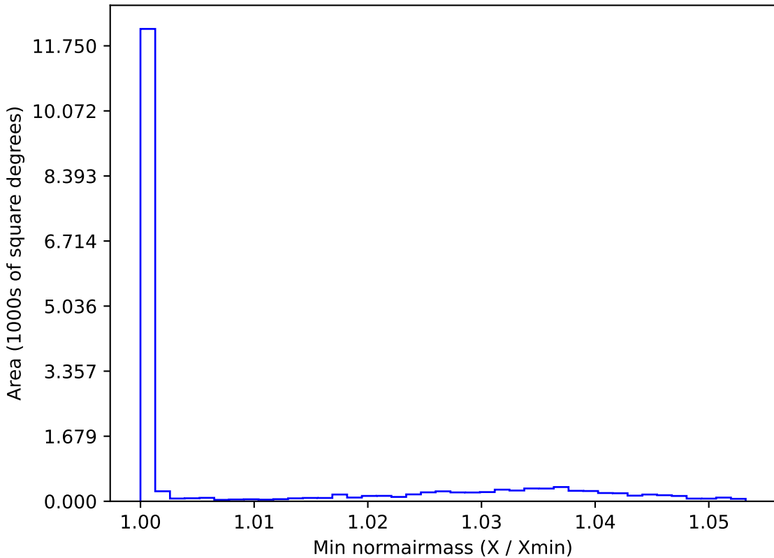
ddf_loaded_fl4_v3.4_10yrs WFD u band: Min normairmass
