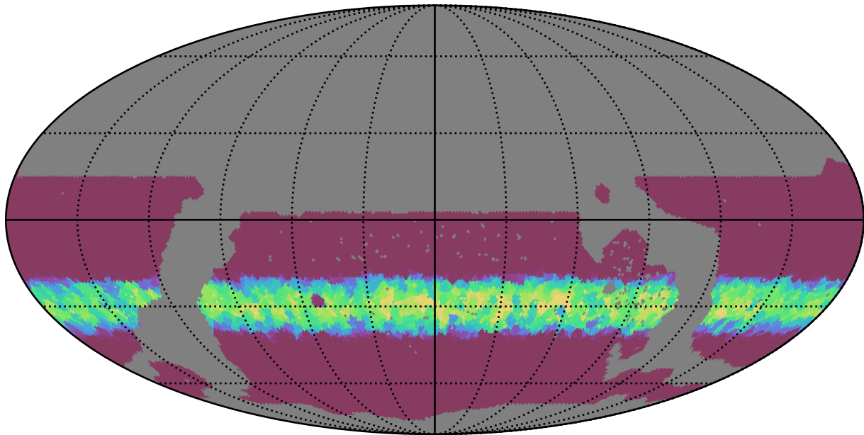
ddf_loaded_fl4_v3.4_10yrs WFD r band: Min normairmass
