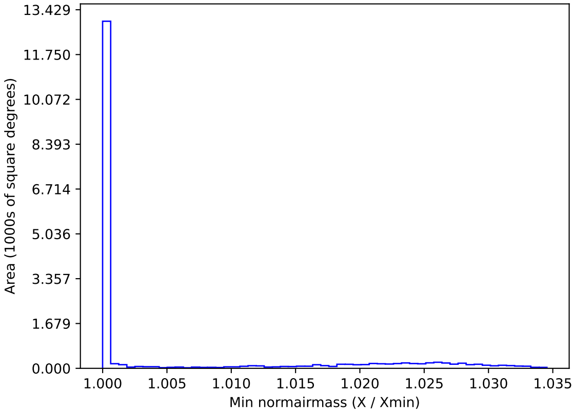
ddf_loaded_fl4_v3.4_10yrs WFD r band: Min normairmass
