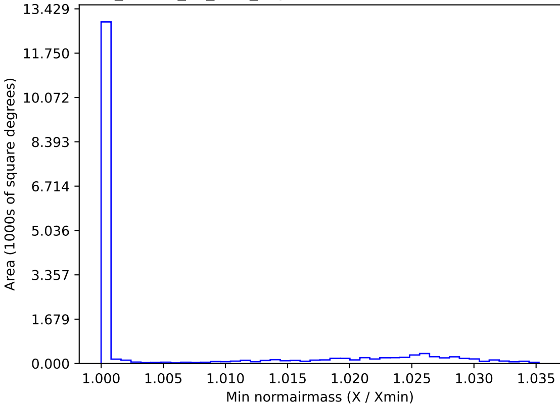
ddf_loaded_fl4_v3.4_10yrs WFD i band: Min normairmass
