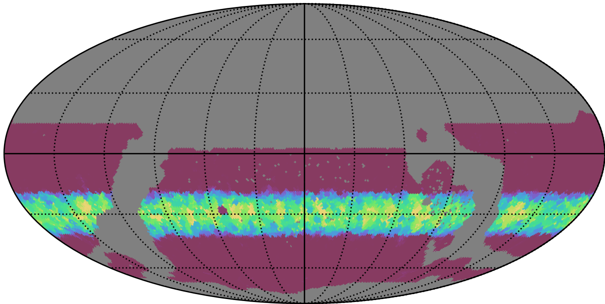
ddf_loaded_fl4_v3.4_10yrs WFD g band: Min normairmass
