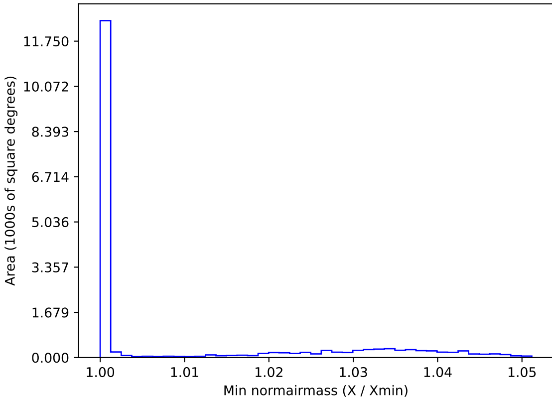
ddf_loaded_fl4_v3.4_10yrs WFD g band: Min normairmass
