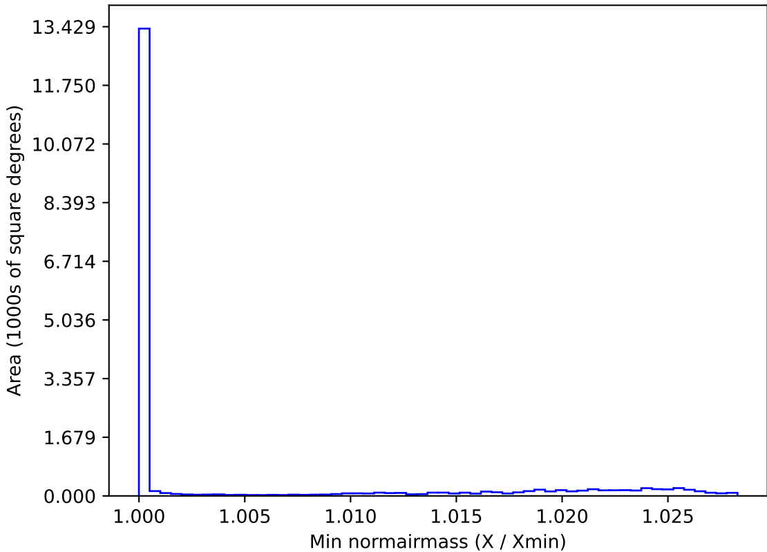
ddf_loaded_fl4_v3.4_10yrs WFD all bands: Min normairmass
