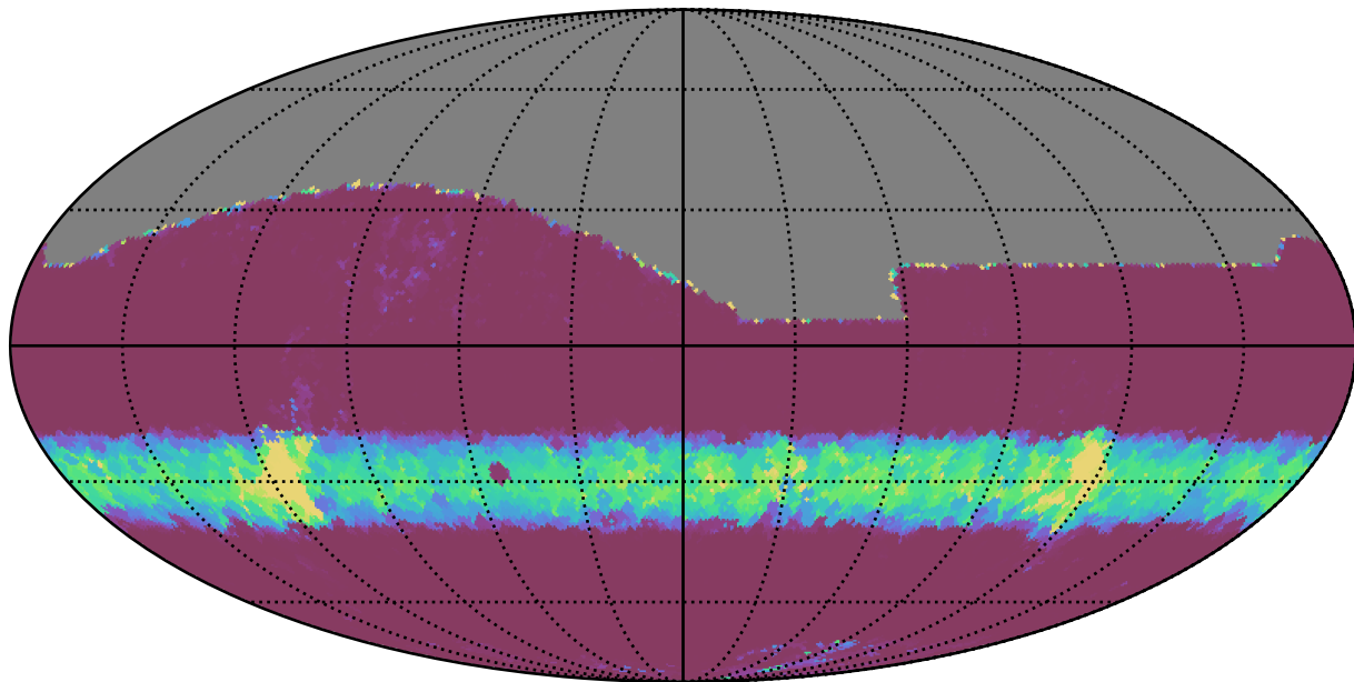
ddf_loaded_fl4_v3.4_10yrs All sky z band: Min normairmass
