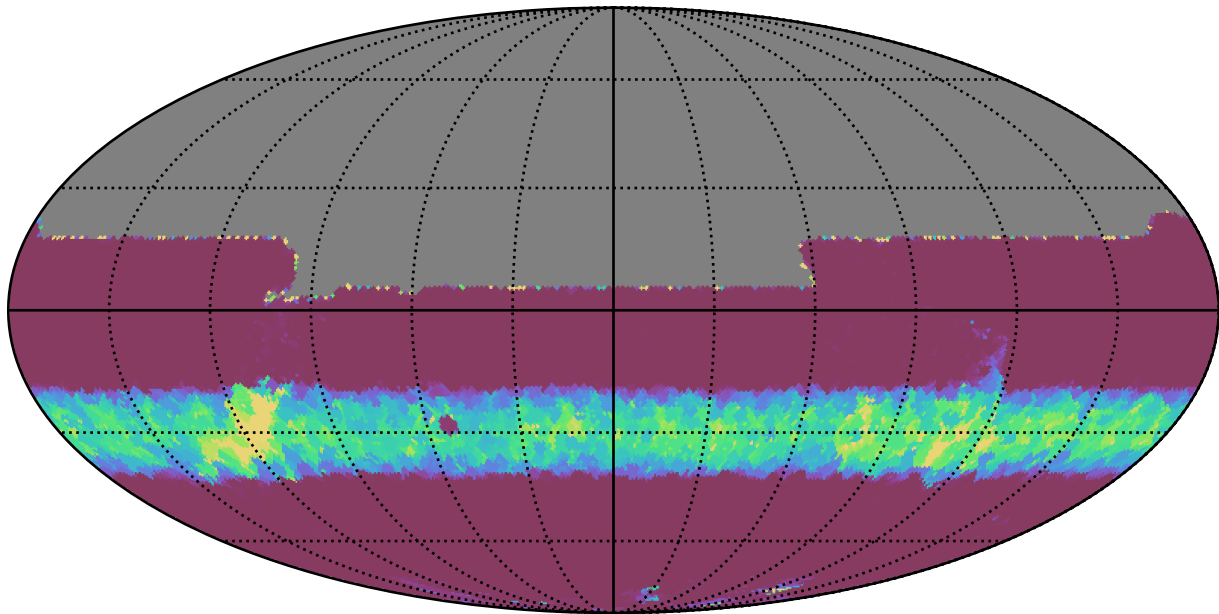
ddf_loaded_fl4_v3.4_10yrs All sky y band: Min normairmass
