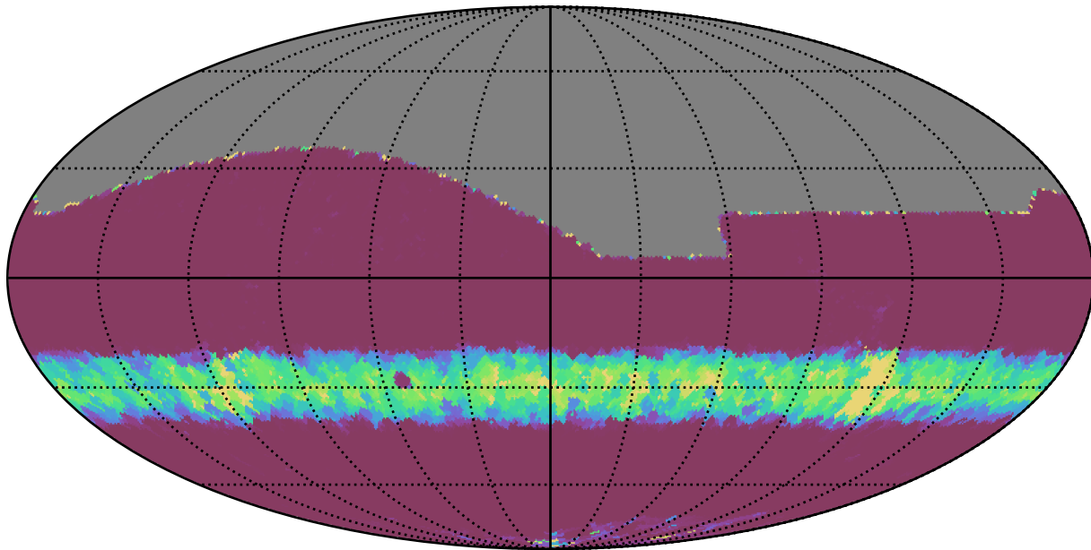
ddf_loaded_fl4_v3.4_10yrs All sky r band: Min normairmass
