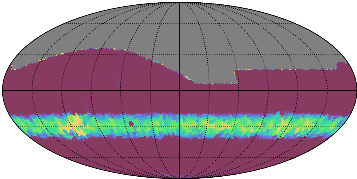
ddf_loaded_fl4_v3.4_10yrs All sky i band: Min normairmass
