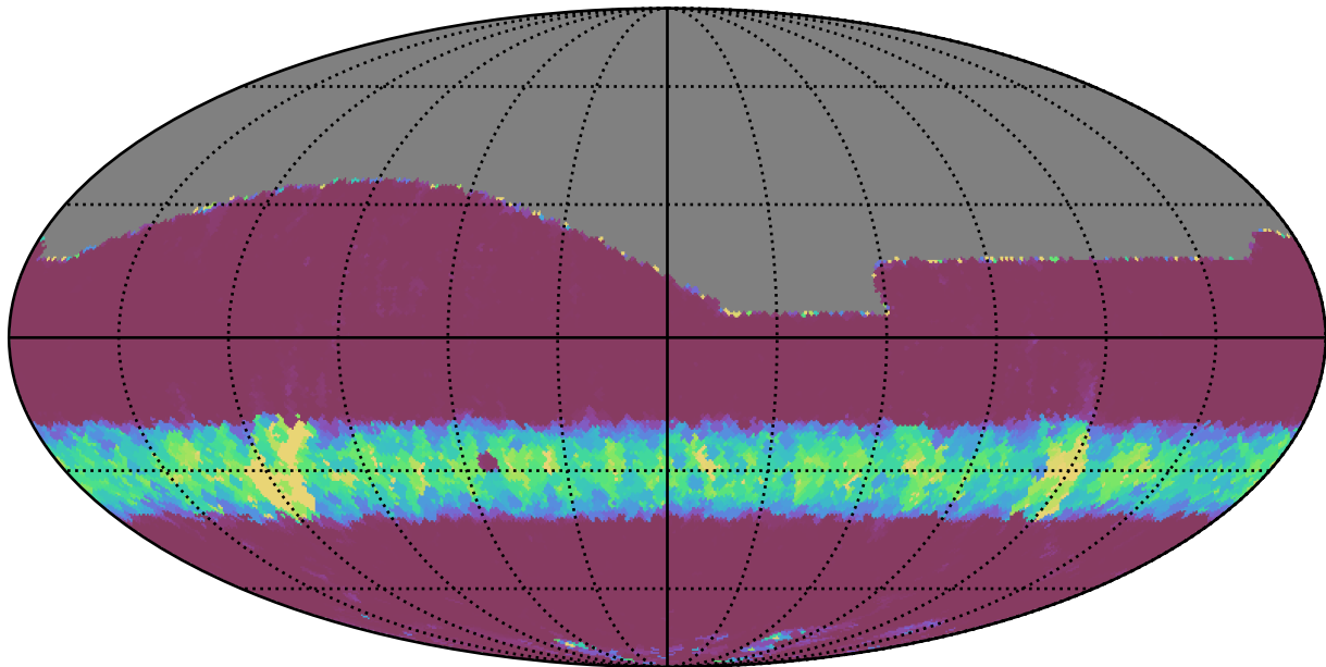
ddf_loaded_fl4_v3.4_10yrs All sky g band: Min normairmass
