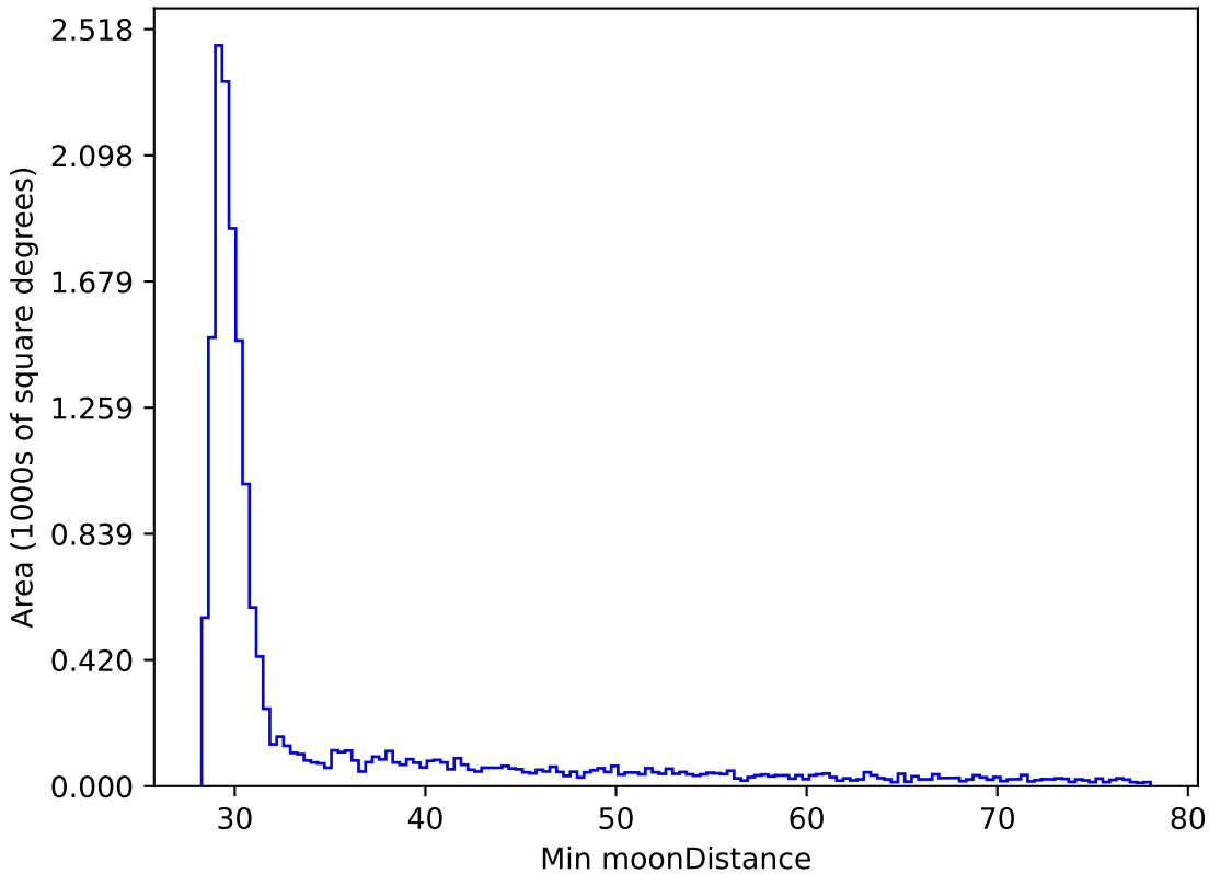
ddf_loaded_fl4_v3.4_10yrs WFD z band: Min moonDistance
