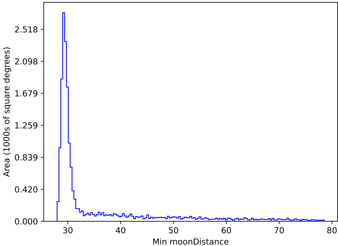
ddf_loaded_fl4_v3.4_10yrs WFD y band: Min moonDistance
