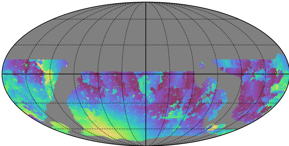
ddf_loaded_fl4_v3.4_10yrs WFD u band: Min moonDistance
