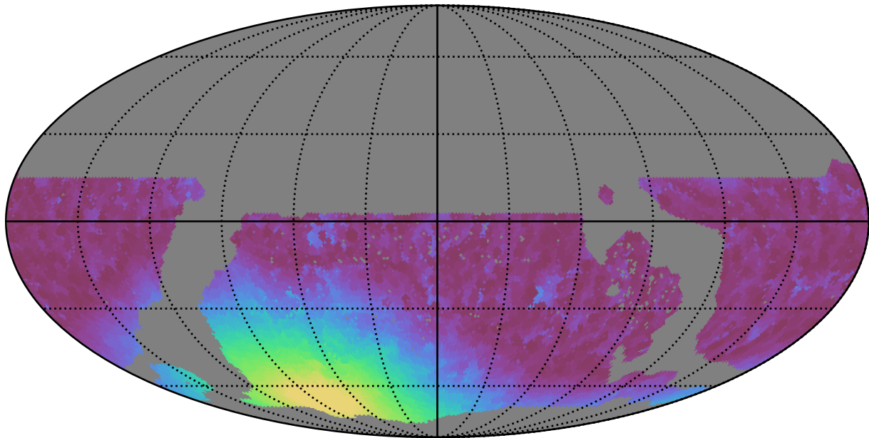
ddf_loaded_fl4_v3.4_10yrs WFD r band: Min moonDistance
