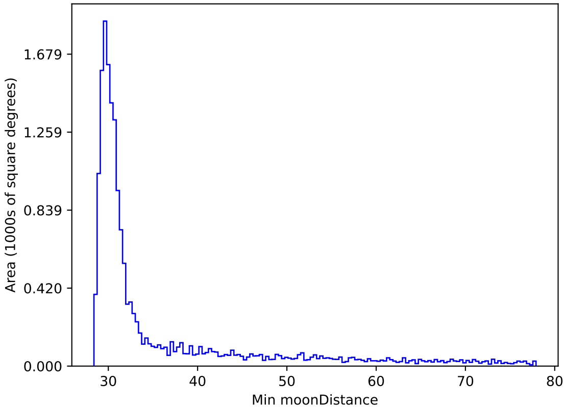
ddf_loaded_fl4_v3.4_10yrs WFD i band: Min moonDistance
