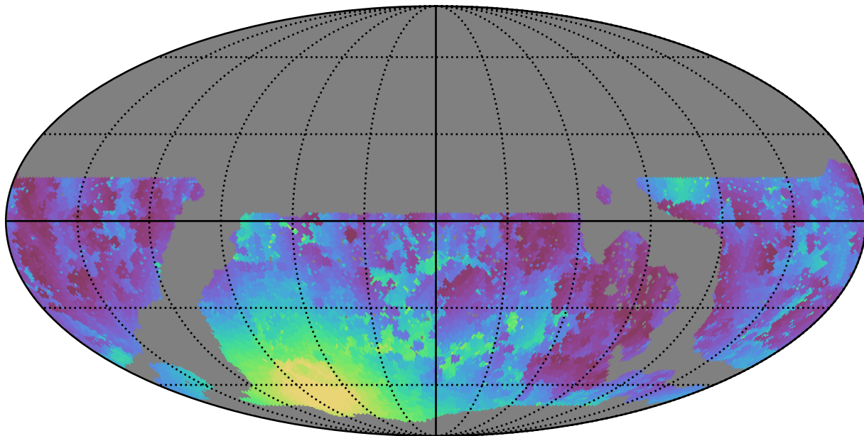
ddf_loaded_fl4_v3.4_10yrs WFD g band: Min moonDistance
