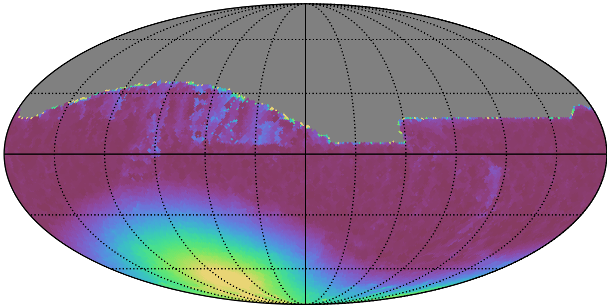
ddf_loaded_fl4_v3.4_10yrs All sky z band: Min moonDistance
