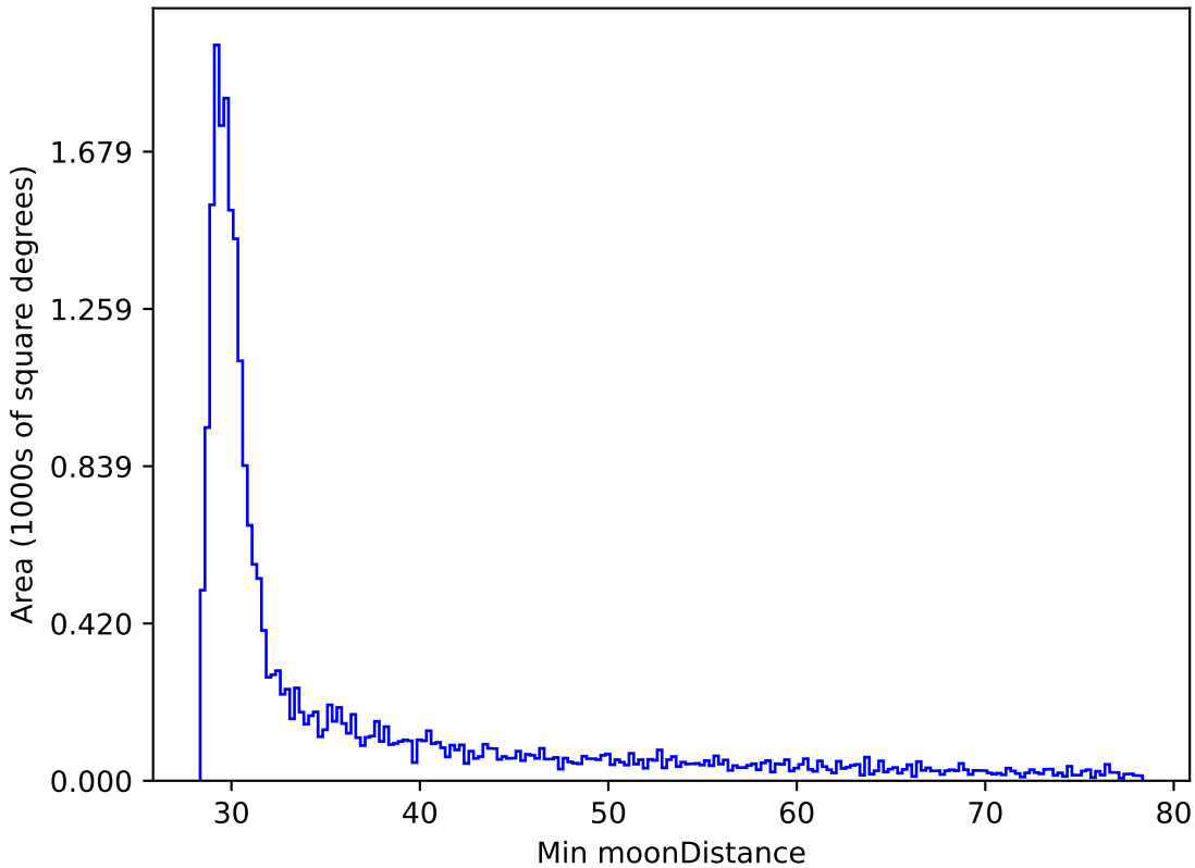
ddf_loaded_fl4_v3.4_10yrs All sky z band: Min moonDistance
