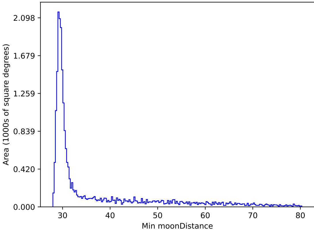
ddf_loaded_fl4_v3.4_10yrs All sky y band: Min moonDistance
