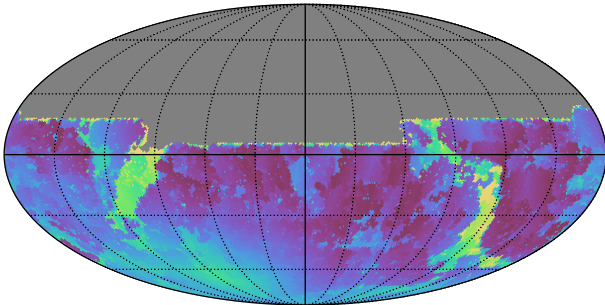
ddf_loaded_fl4_v3.4_10yrs All sky u band: Min moonDistance
