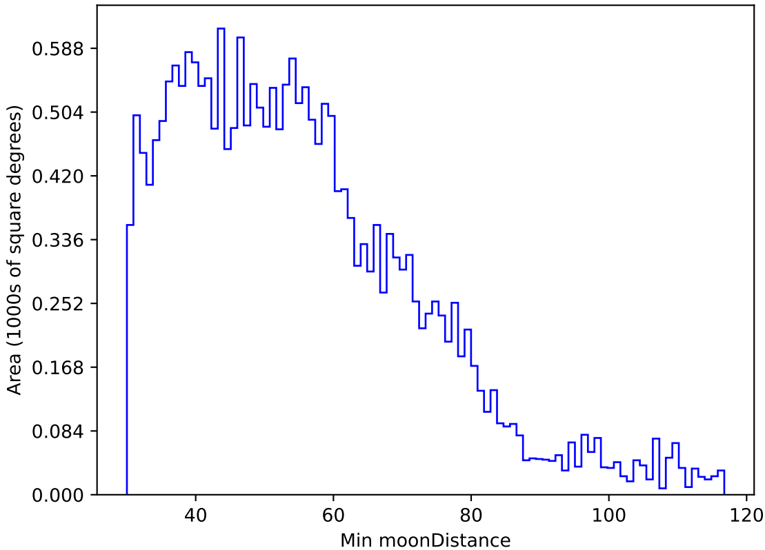
ddf_loaded_fl4_v3.4_10yrs All sky u band: Min moonDistance
