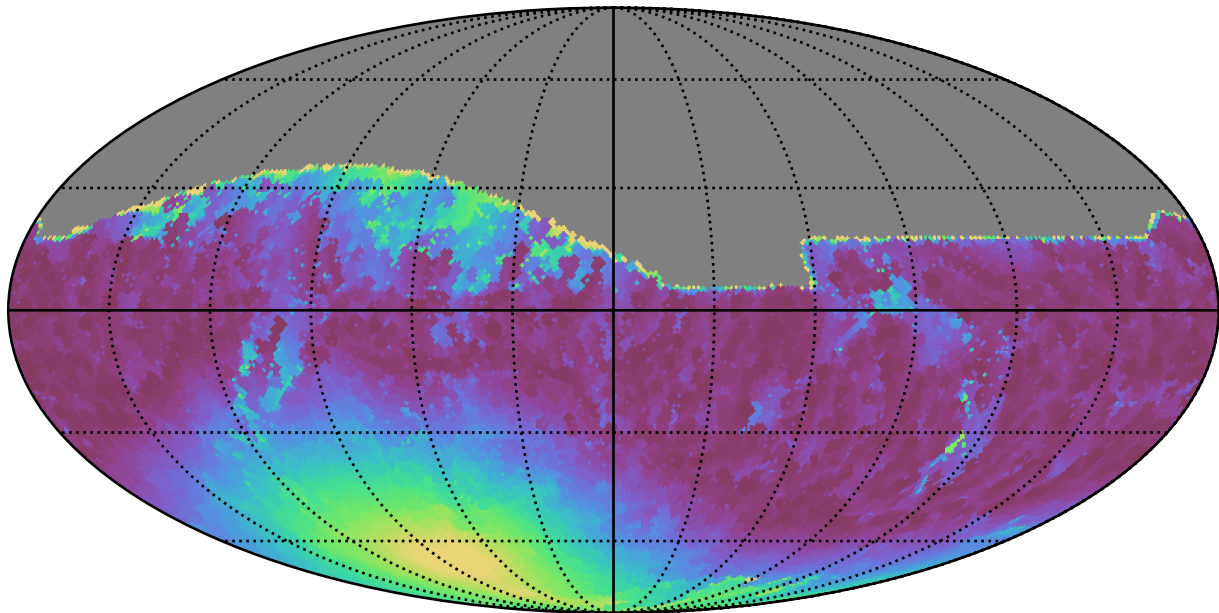
ddf_loaded_fl4_v3.4_10yrs All sky r band: Min moonDistance
