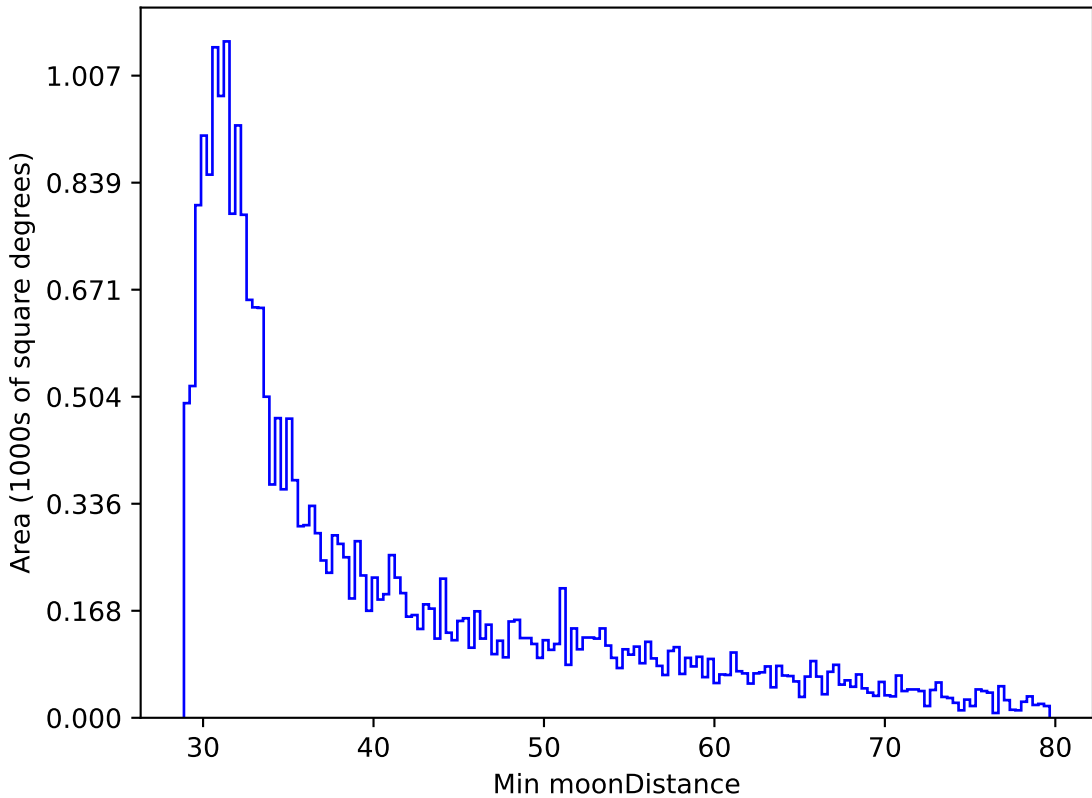
ddf_loaded_fl4_v3.4_10yrs All sky r band: Min moonDistance
