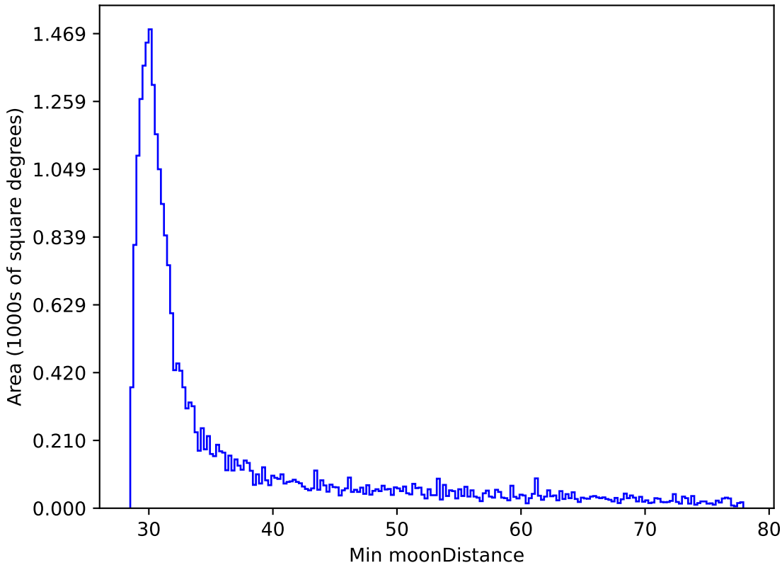
ddf_loaded_fl4_v3.4_10yrs All sky i band: Min moonDistance
