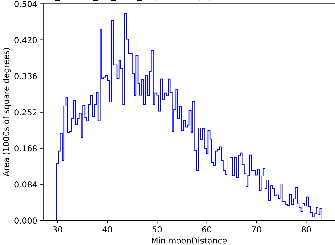
ddf_loaded_fl4_v3.4_10yrs All sky g band: Min moonDistance
