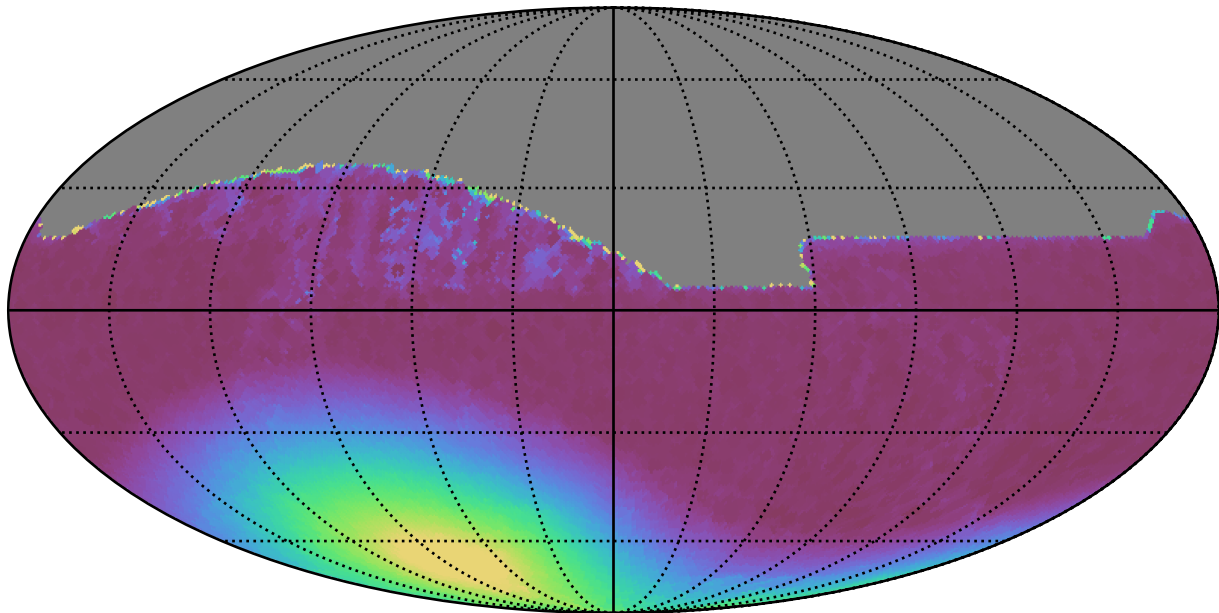
ddf_loaded_fl4_v3.4_10yrs All sky all bands: Min moonDistance
