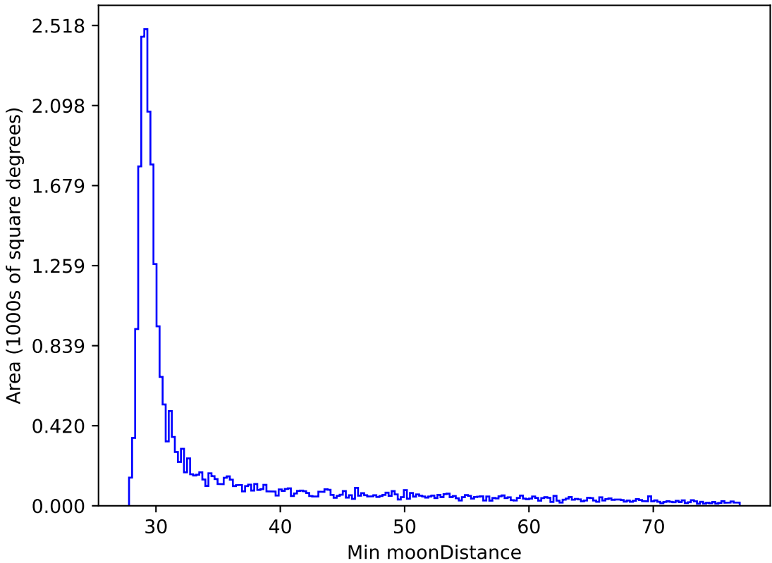
ddf_loaded_fl4_v3.4_10yrs All sky all bands: Min moonDistance
