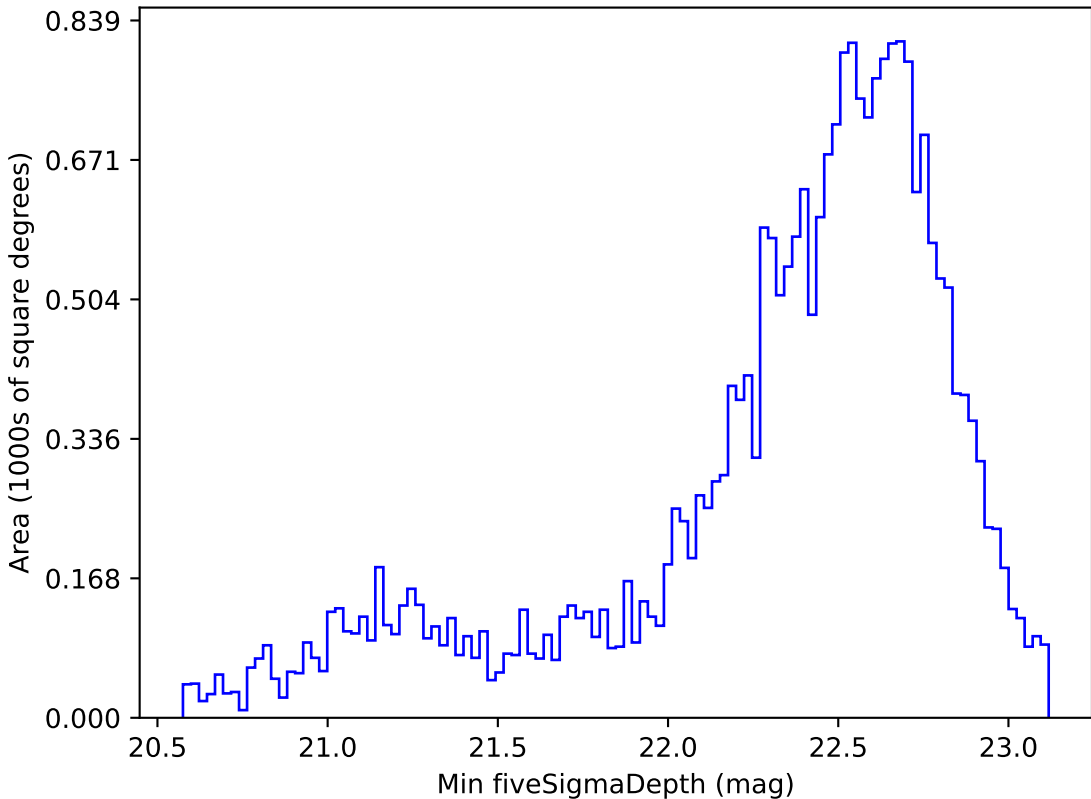
ddf_loaded_fl4_v3.4_10yrs Yr 1 z band: Min fiveSigmaDepth
